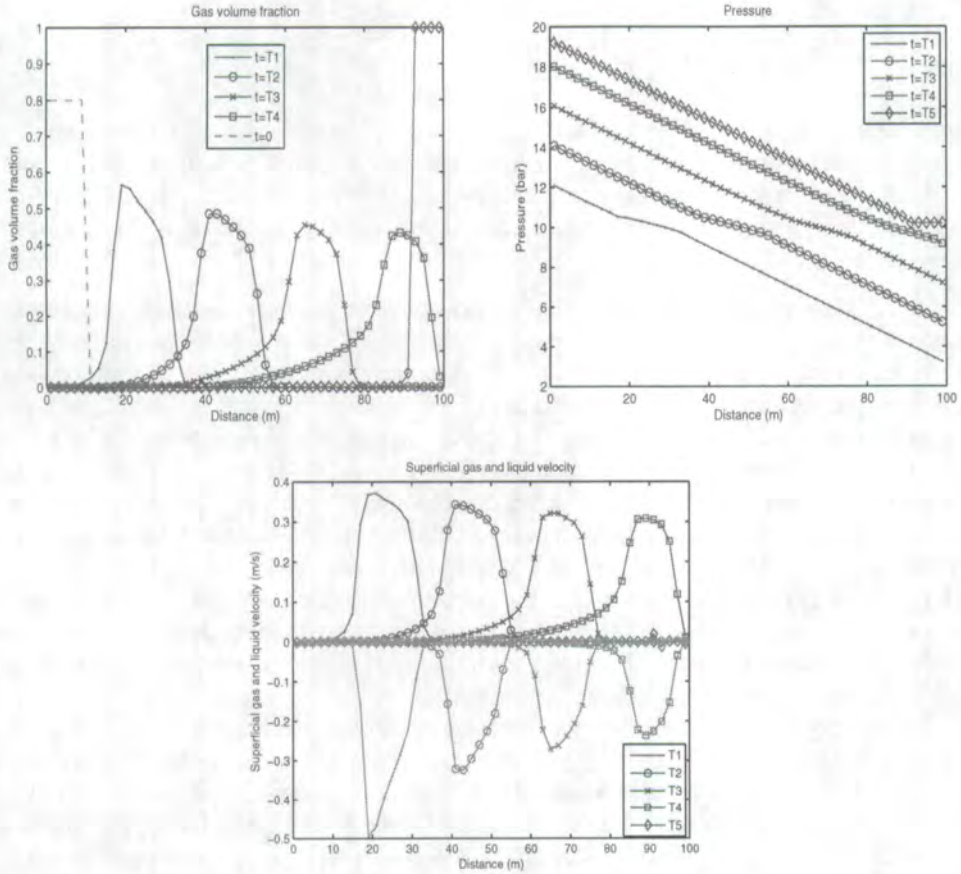
FIG. 1. Top: The behavior of the gas slug (left) and corresponding pressure (right) as the gas slug is moving upwards. Note the increase in pressure as the gas slug is ascending towards the top. Bottom: The superficial velocity of gas ( \alpha_g v_g ) (positive) and liquid ( \alpha_l v_l ) (negative), respectively, reflect the upward movement of the gas slug and the downward behavior of the surrounding liquid. Note that this problem is relatively complicated to solve as it involves strong nonlinear phenomena associated with counter-current flow and challenges associated with transition from two-phase to single-phase flow.
