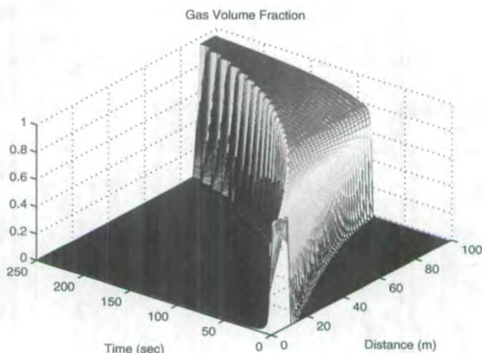
FIG. 4. A visualization of the gas volume fraction in x - t plan. The plot shows the strong expansion effect as the slug is approaching the surface.
