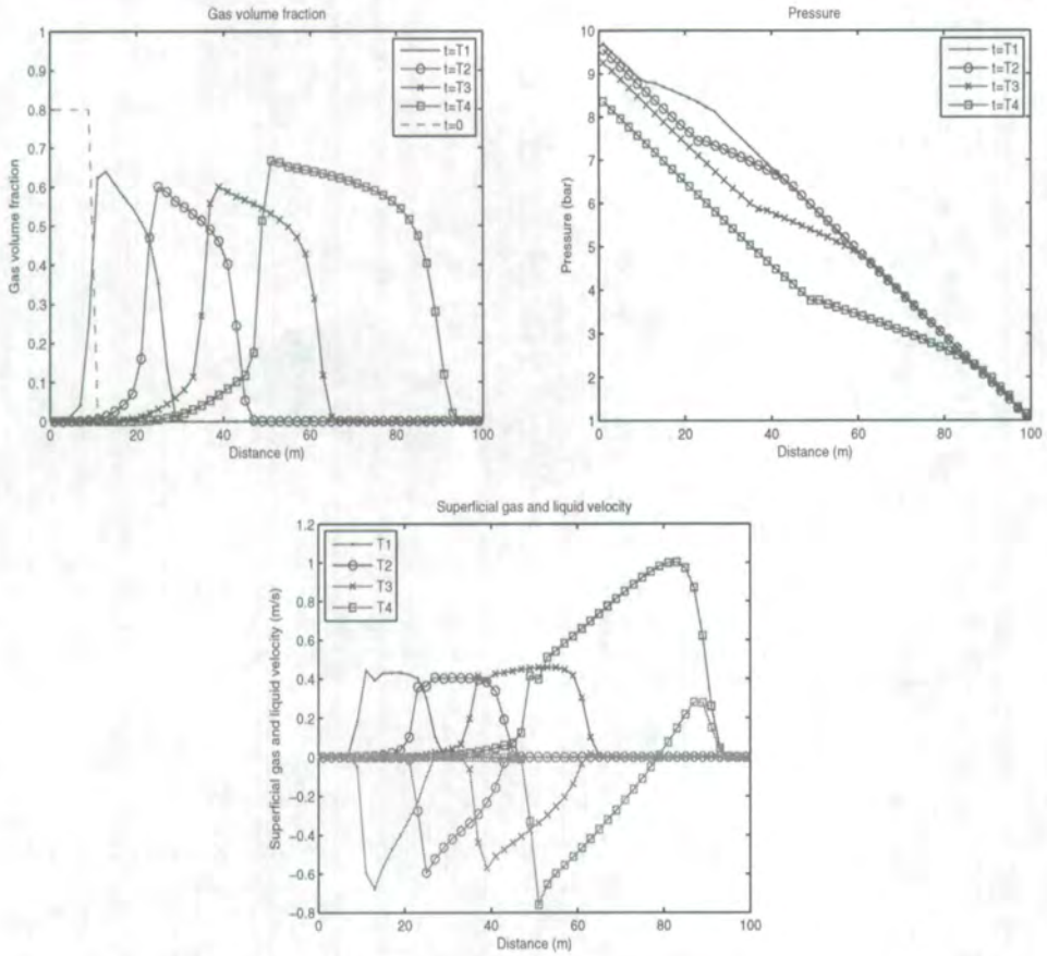
FIG. 3. Top: The gas volume fraction (left plot) reflects the strong expansion effect as the gas slug is approaching the surface where the pressure is equal to ambient pressure. Note the drop in pressure (right plot) as the gas slug is approaching the top. Note also the viscous effect associated with the falling film of liquid that surrounds the gas slug that leads to a lower pressure gradient locally in the slug region. Bottom: The strong expansion of gas close to the open top leads to a strong increase in the gas and liquid superficial velocities.
