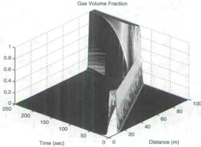
FIG. 2. A visualization of the gas volume fraction in x - t plan. The plot shows the linear trend associated with the ascension velocity of the gas slug. Ultimately, all the gas will be localized in a pure single-phase gas region at the top since the well is closed.
