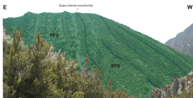
FIGURE 3 | Oblique photograph of the uppermost part of the western limb looking south. It shows an internal unconformity of Guara limestone Fm. that separates the Pre-Folding Sequence (PFS) and the Syn-Folding sequence (SFS). Note how the horizons of the SFS clearly thin towards the E.
