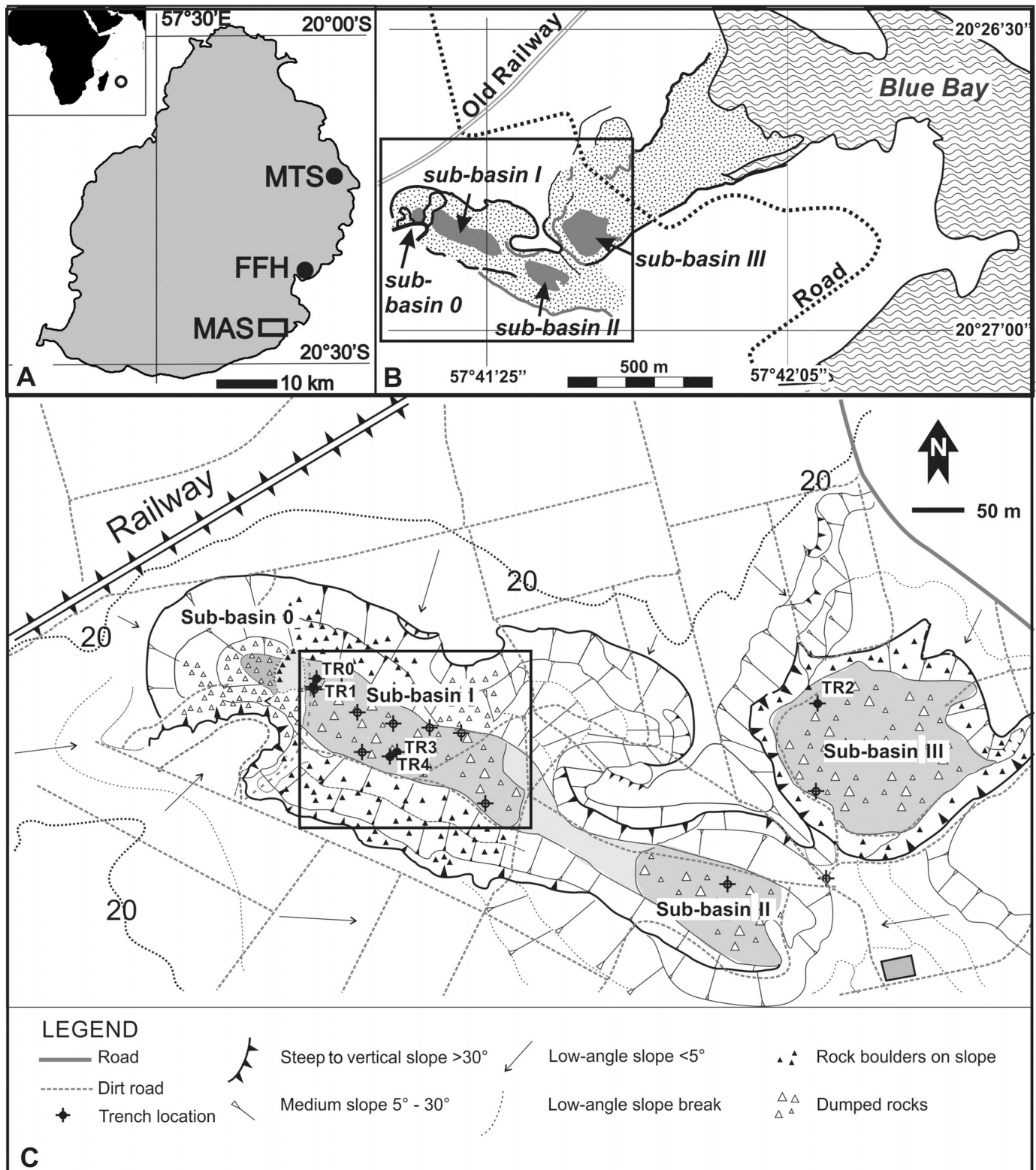
FIGURE 2. A , location of Mauritius in the southwestern Indian Ocean and locations of Mare aux Songs (MAS), Fort Frederik Hendrik (FFH), and Lake Tatos (MTS); B , map of Mare aux Songs and the sub-basins near the coast. Rectangular frame shows extent of inset C ; C , geomorphological map of the Mare aux Songs area showing positions of all sub-basins (0, I, II, III) and locations of trenches TR1 (TR0), TR2, and TR3 (TR4). Rectangular frame shows extent of inset D ; D , left panel showing extent of marsh at sub-basin I. The dashed line represents the longitudinal cross-section with positions of dated and undated samples from cores, scoops, and trenches. Right panel showing the longitudinal cross-section through the marsh with locations of radiocarbon dated samples (see Table 1). B is carbonate sands, C is lake marl and gyttja, D is fossil layer, and E is dumped basalt boulder layer.
