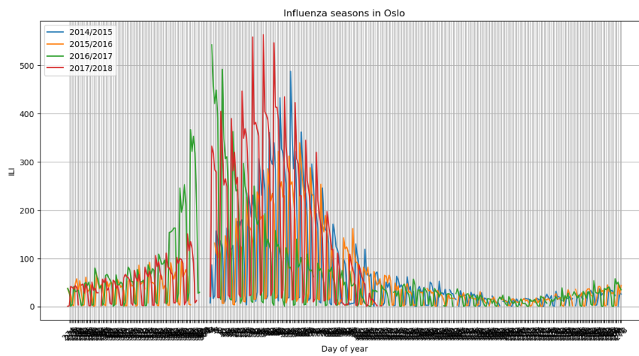
Figure 4.6: Influenza-like illnesses season 2014-2018 in Oslo
