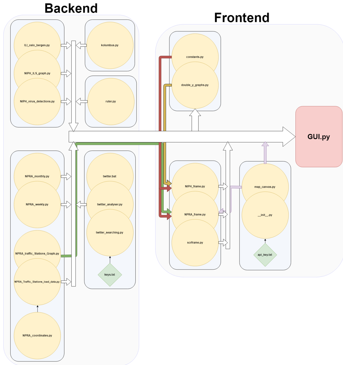
Figure 4.2: Simplification of the overall program structure and relation
