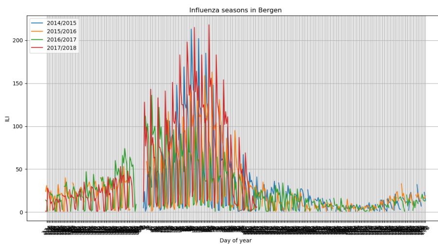
Figure 4.7: Influenza-like illnesses season 2014-2018 in Bergen
