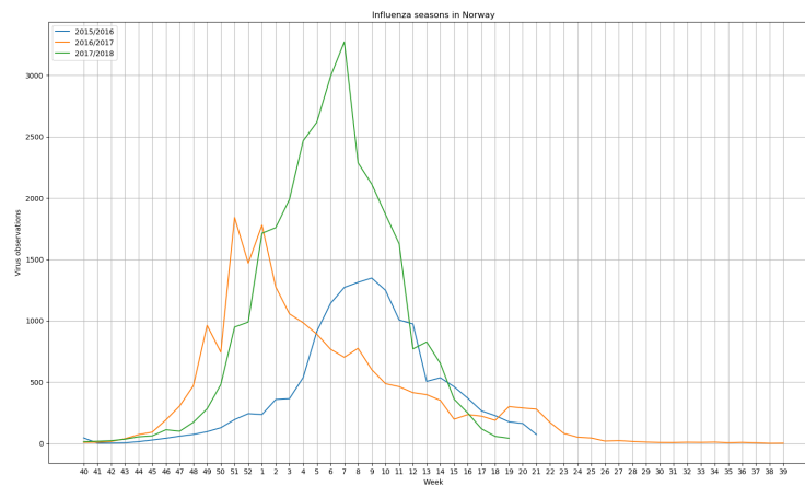
Figure 4.4: Influenza virus observation
