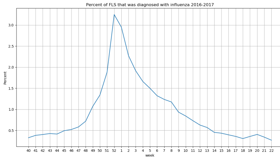
Figure 4.5: Influenza-like illnesses season 2016/2017
