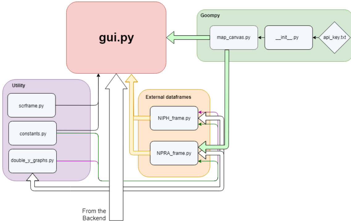
Figure 4.18: A semi detailed diagram of the Frontend structure and functions
