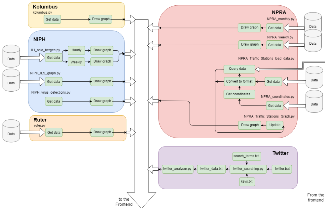
Figure 4.3: A semi detailed diagram of the Backend structure and functions
