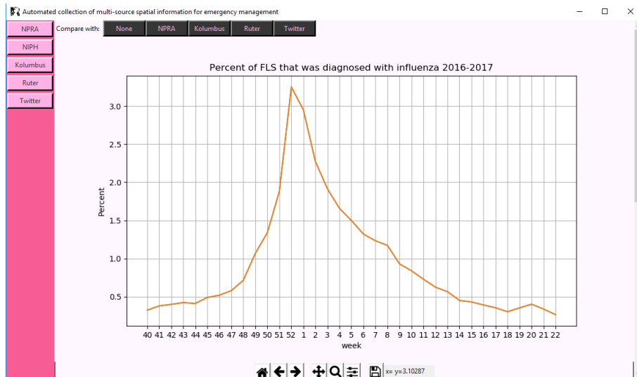
Figure 4.19: The GUI
