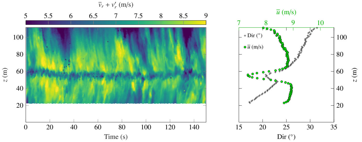
Figure 6: Left: Radial wind velocity recorded by R2D1 during the vertical scan on 23/05/2014 from 05:30. Right: Vertical profiles of the mean wind velocity and the mean wind direction evaluated using the lidars measurements between 05:30 and 05:40.
