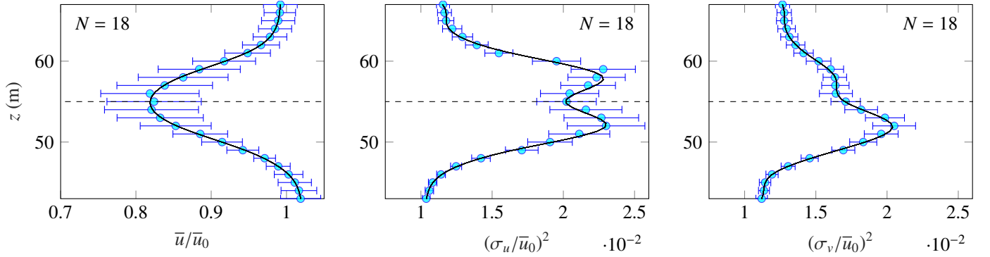
Figure 10: Vertical profiles of the mean wind velocity and standard deviation of the wind velocity from 43 m to 67 m, corresponding to 0.08 \leq I_u \leq 0.14 and 5.2 \text{ m s}^{-1} \leq \bar{u} \leq 9.8 \text{ m s}^{-1} at z = 67 \text{ m} and z = 43 \text{ m} . The averaged data are displayed as a scatter plot with horizontal errorbars representing two standard deviations. The solid black line is a piecewise cubic spline (—) fitted to the averaged data. The position of the deck centre is indicated by a horizontal dashed line (- -) and the number of samples used is denoted N .
