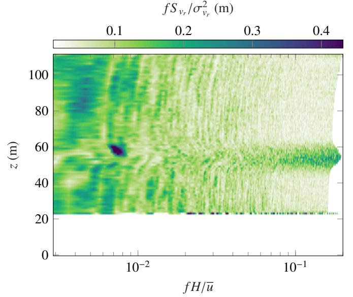
Figure 13: Normalized along-beam wind velocity spectrum estimated using wind data recorded from 01:00 to 07:50 on 23/05/2014 with \bar{v}_r(z = 65 \text{ m}) \geq 5 \text{ m s}^{-1} (19 samples), at each measurement height along the vertical line scanned by the WindScanner system.
