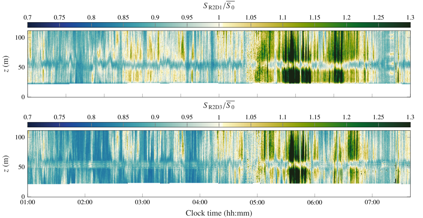
Figure 5: Evolution of the ratios S_{R2D3}/\overline{S_0} and S_{R2D1}/\overline{S_0} with the measurement height and the time for the lidar R2D1 (top) and R2D3 (bottom) on 23/05/2014, where S_{R2D1} and S_{R2D3} are the NDSM of the lidar R2D1 and R2D3, respectively; \overline{S_0} is the NDSM of the lidar R2D1 averaged over the measurement period and the measurement height.
