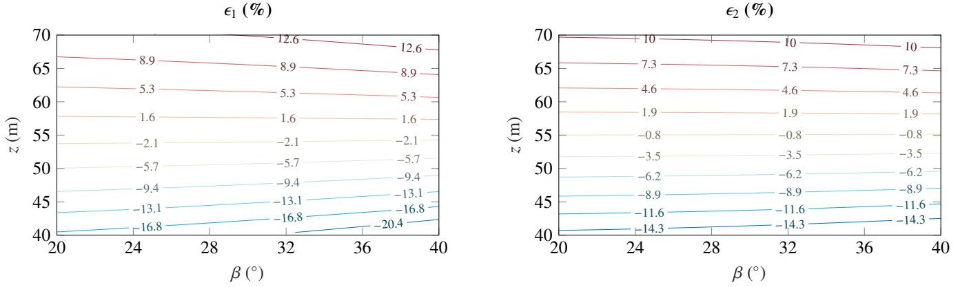
Figure 4: Error induced on the RMS of the along-beam wind velocity at each lidar by disregarding the vertical wind component.
