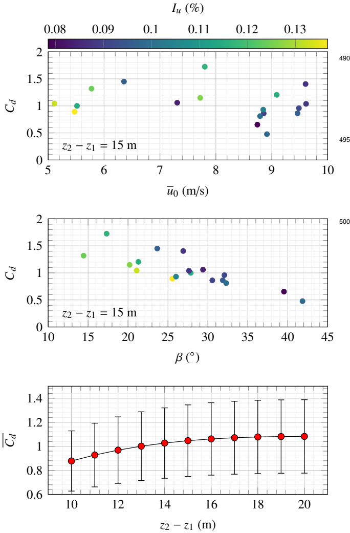
Figure 11: Drag coefficient calculated for wind data recorded on 23/05/2014 from 01:00 to 07:50, expressed as a function of the undisturbed mean wind velocity (top) or the yaw angle (middle). The bottom panel shows the dependency of the averaged drag coefficient on the wake width.
