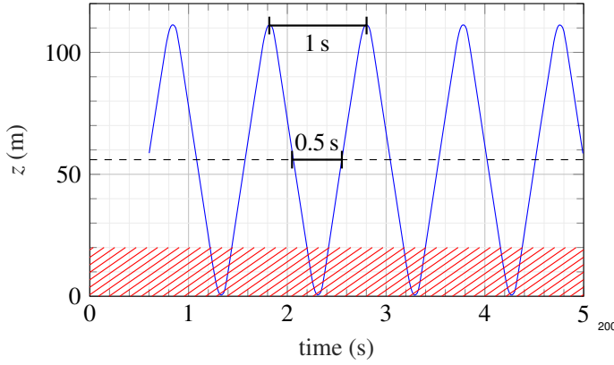
Figure 3: First five seconds of the trajectory (solid line) of the scanning volume. The dashed line corresponds to the height at which the lidars are located: The hatched area denotes the domain that is not reached by the beams, due to their intersection with the deck.
