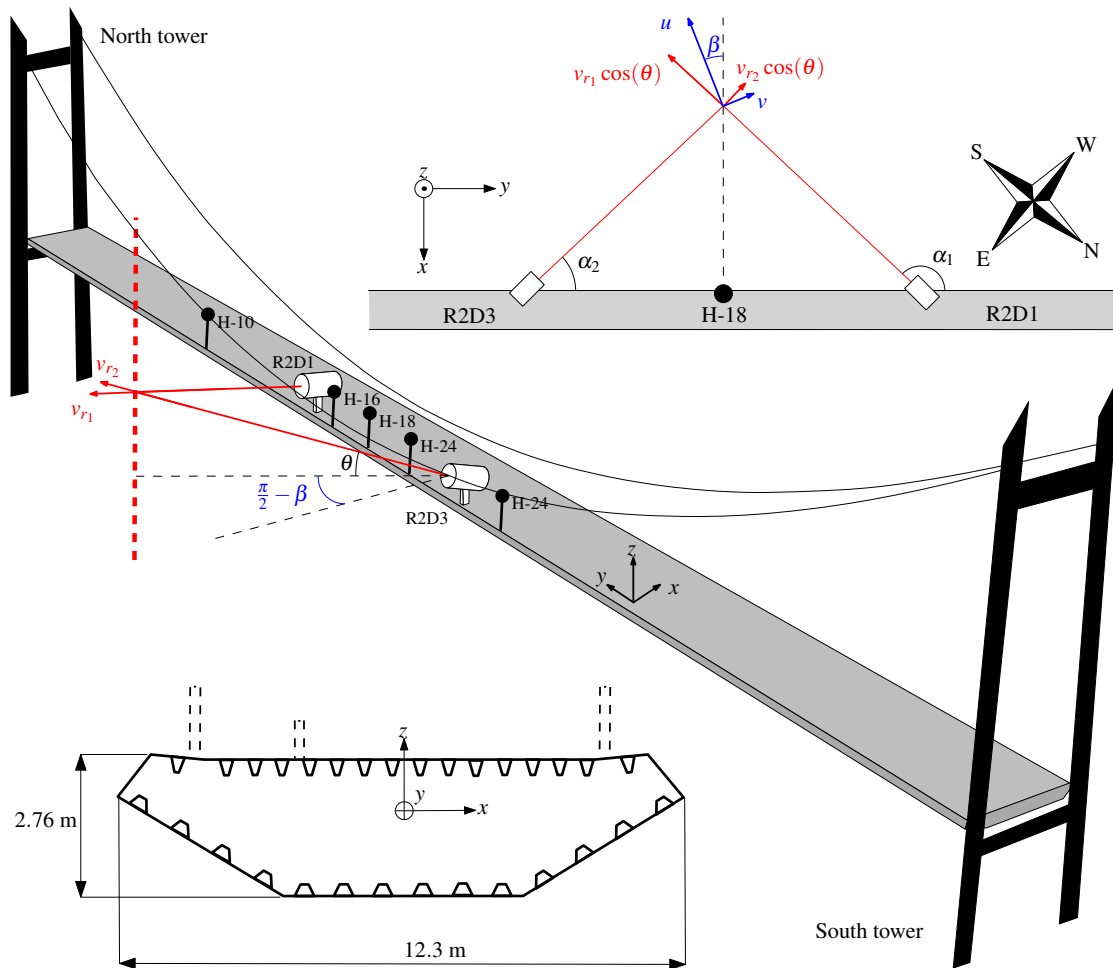
Figure 2: Schematic of the dual-lidar scanning system (R2D1 and R2D3) monitoring the flow near H-18. Hangers are not drawn and the scales are not respected for the sake of clarity.
