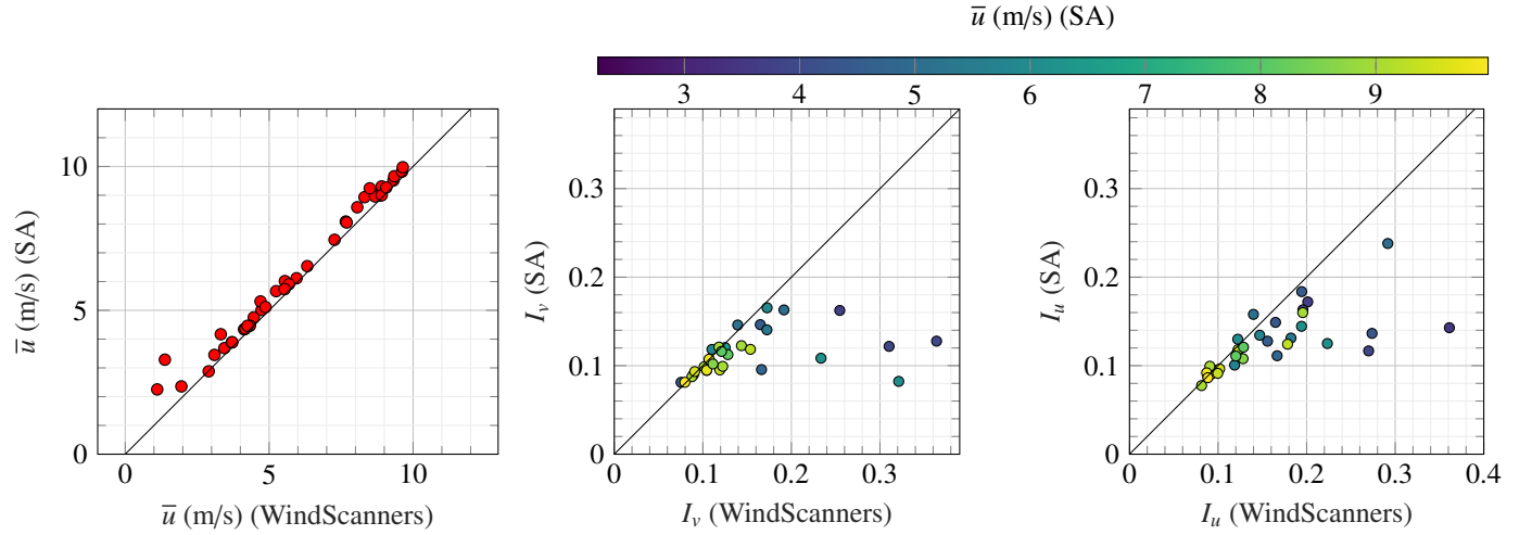
Figure 9: Mean wind velocity (left panel), crosswind turbulence intensity (middle panel) and along-wind turbulence intensity (right panel) recorded by the WindScanners 65 m above the sea level (horizontal axis), 40 m downstream of the deck, compared to the sonic anemometer (SA) measurements on H-18 (vertical axis). The data used corresponds to the record period spanning from 01:00 to 07:50 on 23/05/2014.
