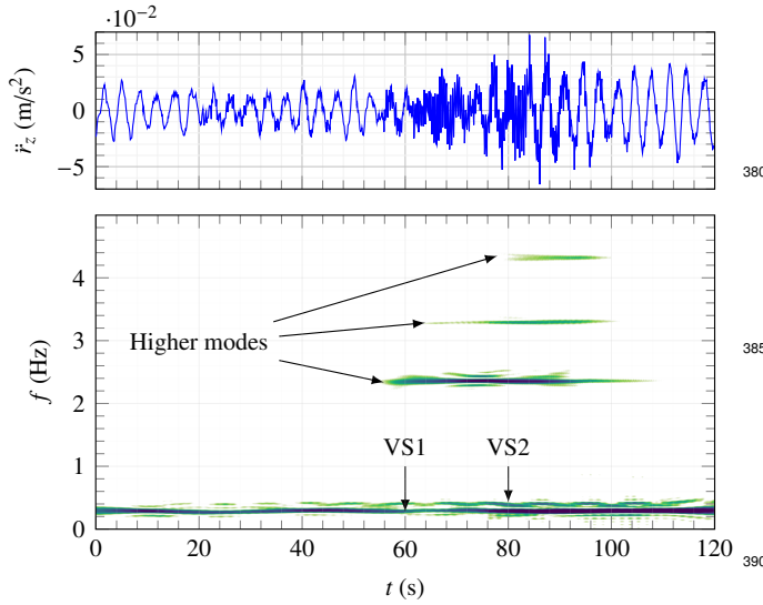
Figure 8: Vertical bridge acceleration at midspan (top) and corresponding normalized EPSPD (bottom) from 05:30:00 on 23/05/2014.
