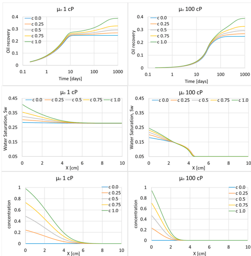
Fig. 11. Secondary imbibition enhanced oil recovery where brine with WA component imbibes from initial time for different concentrations. The left figures indicate cases with oil viscosity of 1 cP, while right figures indicate cases with 100 cP oil viscosity. A capillary back pressure of 1 bar was assumed to eliminate counter-current production. RF^{co} = RF^{tot} is displayed in row 1. Water saturation profiles and concentration profiles after 10 d are shown in row 2 and row 3, respectively.
