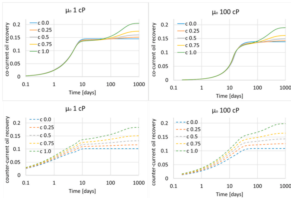
Fig. 9. Secondary imbibition enhanced oil recovery where brine with WA component imbibes from initial time for different concentrations. The left figures indicate cases with oil viscosity of 1 cP, while right figures indicate cases with 100 cP oil viscosity. P_{cbo} = 0 was assumed. Co-current recovery RF^{co} (solid lines) and counter-current recovery RF^{cc} (dashed lines) are displayed in row 1 and 2, respectively.
