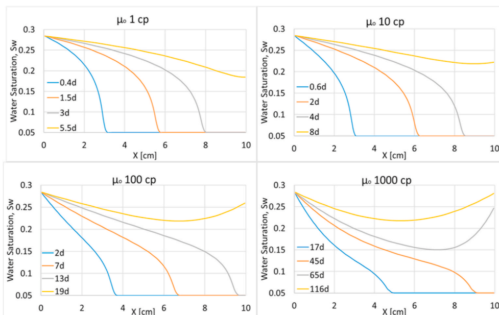
Fig. 5. Water saturation profiles during SI under pow conditions, displayed when RF^{tot} = 0.05 (blue), 0.10 (orange), 0.15 (grey) and 0.20 (yellow) for different oil viscosities. The absolute times are indicated. (For interpretation of the references to color in this figure legend, the reader is referred to the Web version of this article.)
