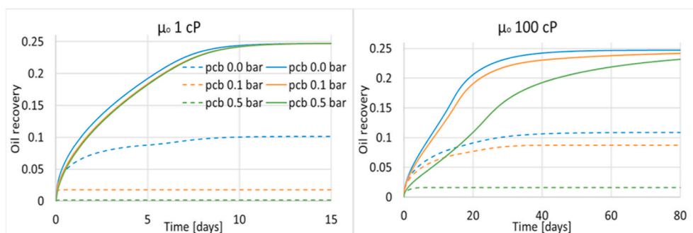
Fig. 7. The effect of capillary back pressure on SI at fixed pow wetting state. The solid lines indicate total recovery, while the dashed lines indicate counter-current recovery.
