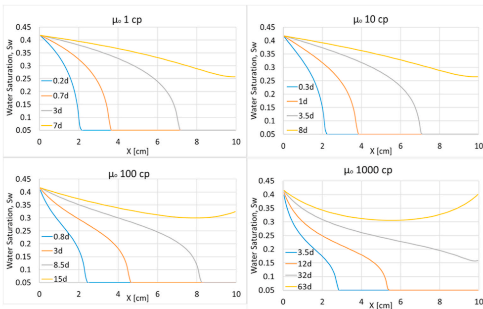
Fig. 6. Water saturation profiles during SI under pww conditions, displayed when RF^{tot} = 0.05 (blue), 0.10 (orange), 0.20 (grey) and 0.30 (yellow) for different oil viscosities. The absolute times are indicated. (For interpretation of the references to color in this figure legend, the reader is referred to the Web version of this article.)
