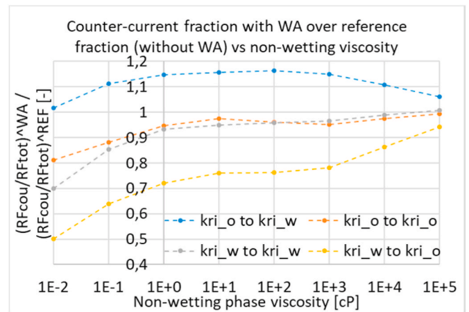
Fig. 16. The ratio \left(\frac{RF_{cou}}{RF_{tot}}\right)^{WA} / \left(\frac{RF_{cou}}{RF_{tot}}\right)^{ref} plotted against viscosity for different shifts in relative permeability during WA.
