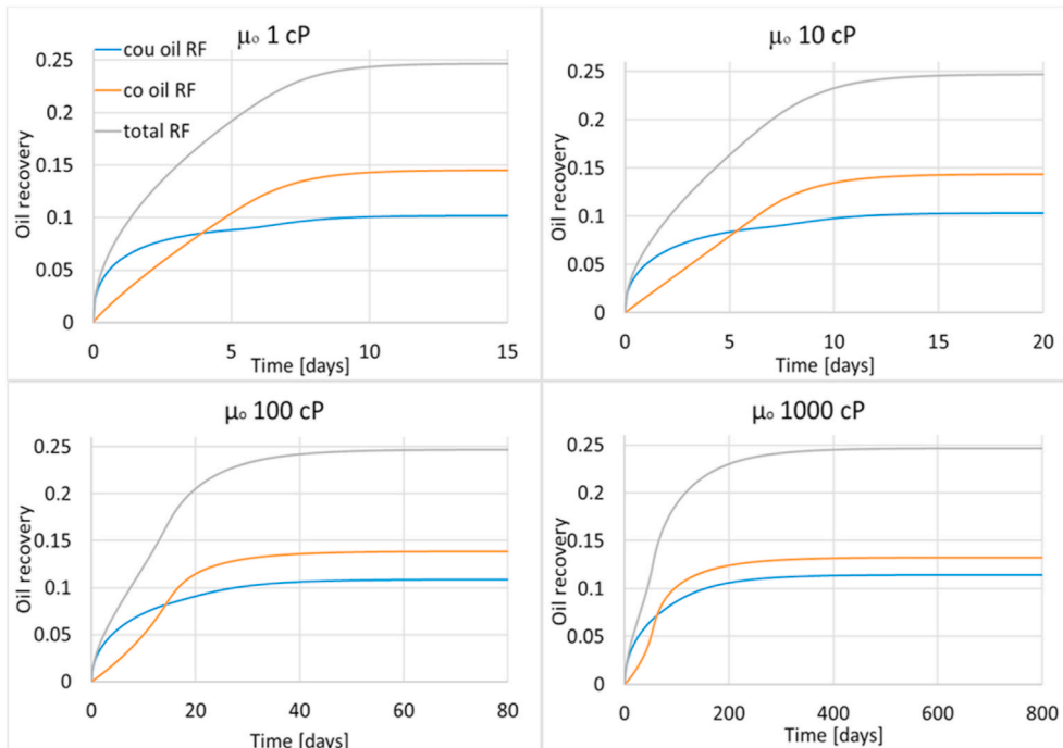
Fig. 3. Recovery vs time at fixed pow state for different oil viscosities. Reference parameters were used.
