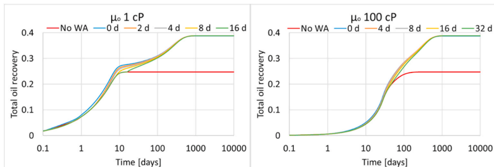
Fig. 14. Tertiary oil recovery for oil viscosity 1 cP (left) and 100 cP (right). A capillary back pressure of 1 bar is assumed to eliminate counter-current production. Initially water imbibes with c = 0 such that pow state remains for some time. At the indicated times brine with concentration c = 1 imbibes. RF^{co} = RF^{tot} is shown.
