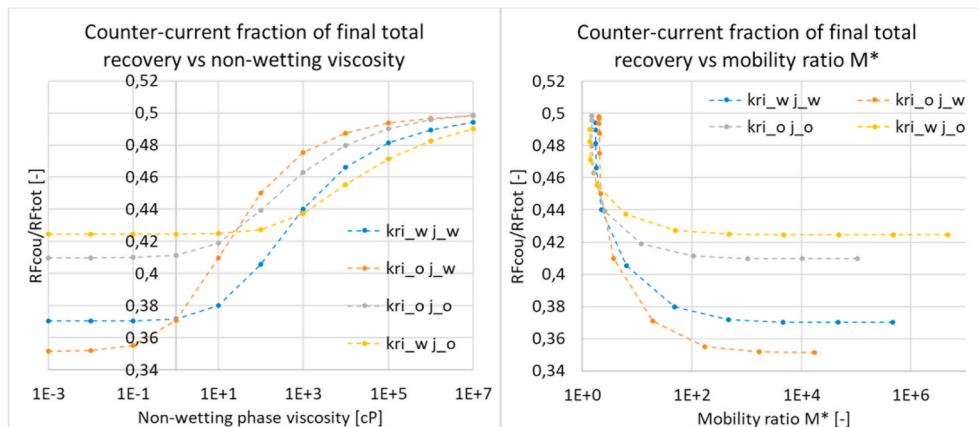
Fig. 15. The fraction of counter-current production out of total production at end of SI plotted against viscosity (left) and mobility ratio M^* (right). The combinations of saturation functions are indicated. Results from simulations are shown as points, while the lines are intended to indicate trends.
