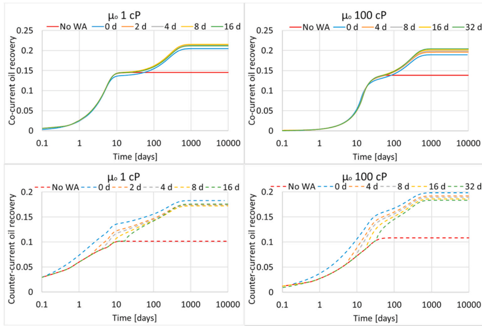
Fig. 13. Tertiary oil recovery for oil viscosity 1 cP (left) and 100 cP (right). Initially water imbibes with c = 0 such that pow state remains for some time. At the indicated times brine with concentration c = 1 imbibes. RF^{co} and RF^{cou} are shown in row 1 and row 2, respectively. Zero capillary back pressure is assumed.
