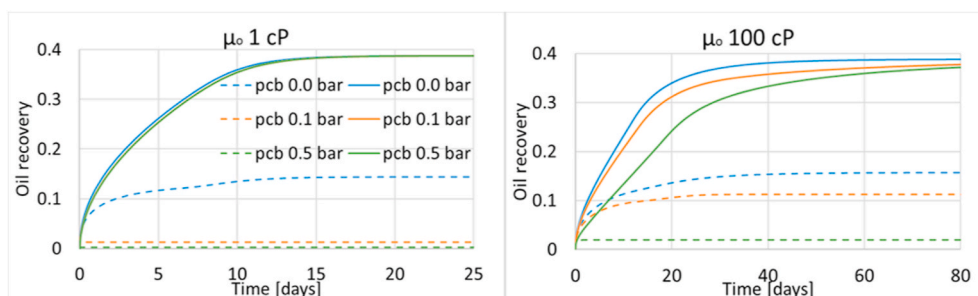
Fig. 8. The effect of capillary back pressure on SI at fixed pww wetting state. The solid lines indicate total recovery, while the dashed lines indicate counter-current recovery.
