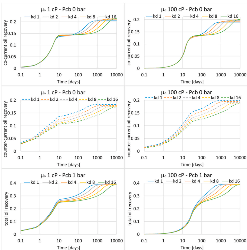
Fig. 12. The role of adsorption distribution coefficient k_d on imbibition behavior for oil viscosity of 1 cP (left) and 100 cP (right) when WA with c = 1 is performed. RF^{co} and RF^{con} are shown in row 1 and 2, respectively, for the case of a zero capillary back pressure. In row 3 a back pressure of 1 bar is assumed and RF^{co} = RF^{tot} is shown (no counter-current production).
