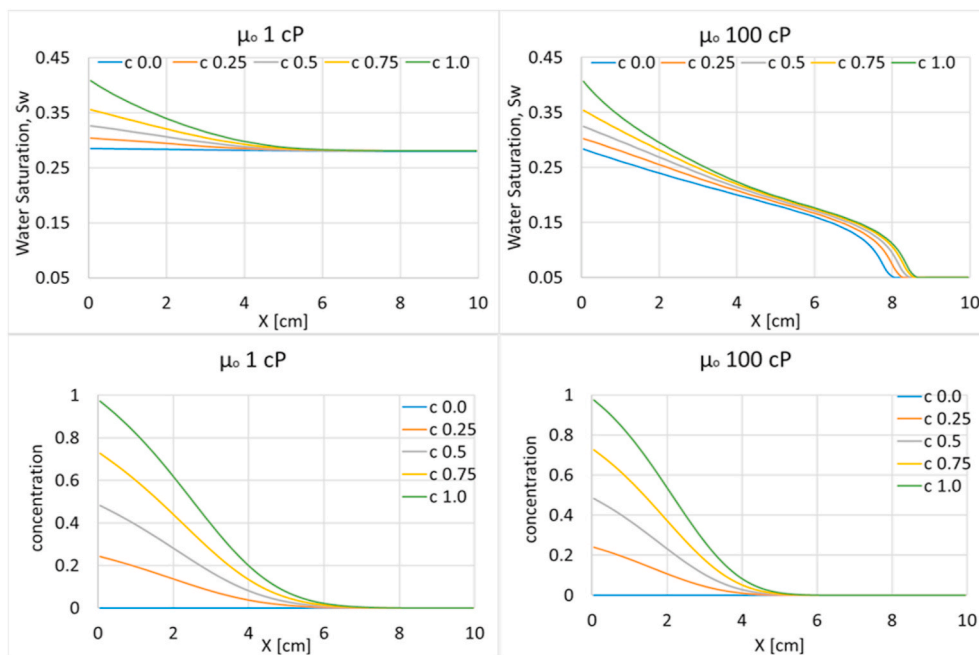
Fig. 10. Secondary imbibition enhanced oil recovery where brine with WA component imbibes from initial time for different concentrations. The left figures indicate cases with oil viscosity of 1 cP, while right figures indicate cases with 100 cP oil viscosity. P_{cbo} = 0 was assumed. Water saturation profiles and concentration profiles after 10 d are shown in row 1 and row 2, respectively.
