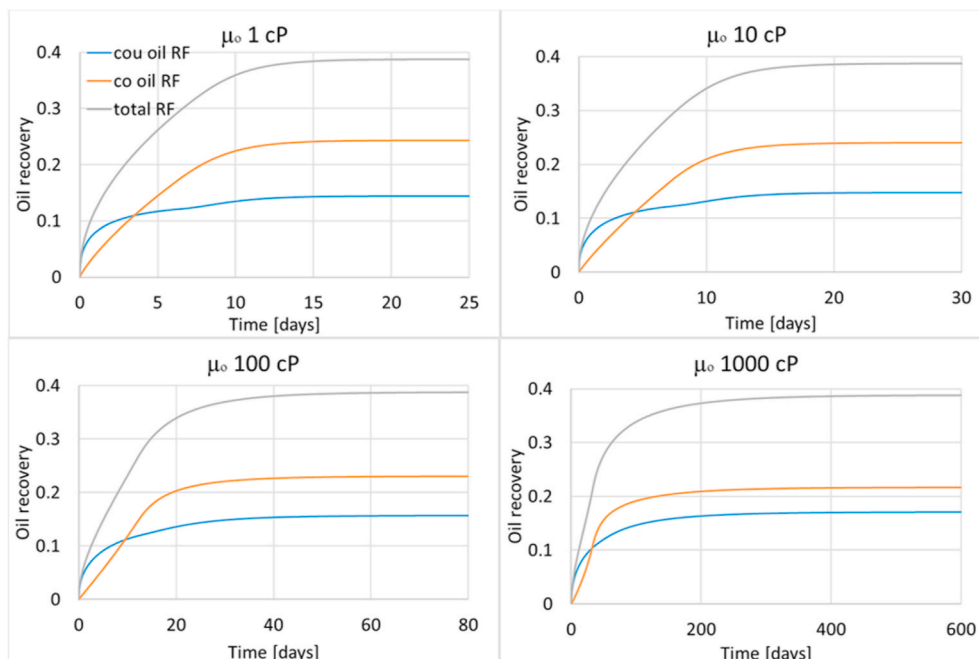
Fig. 4. Recovery vs time at fixed pww state for different oil viscosities. Reference parameters were used.
