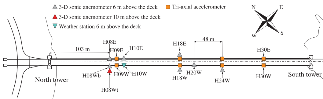
FIGURE 1 Instrumentation of the Lysefjord Bridge since July 2017
