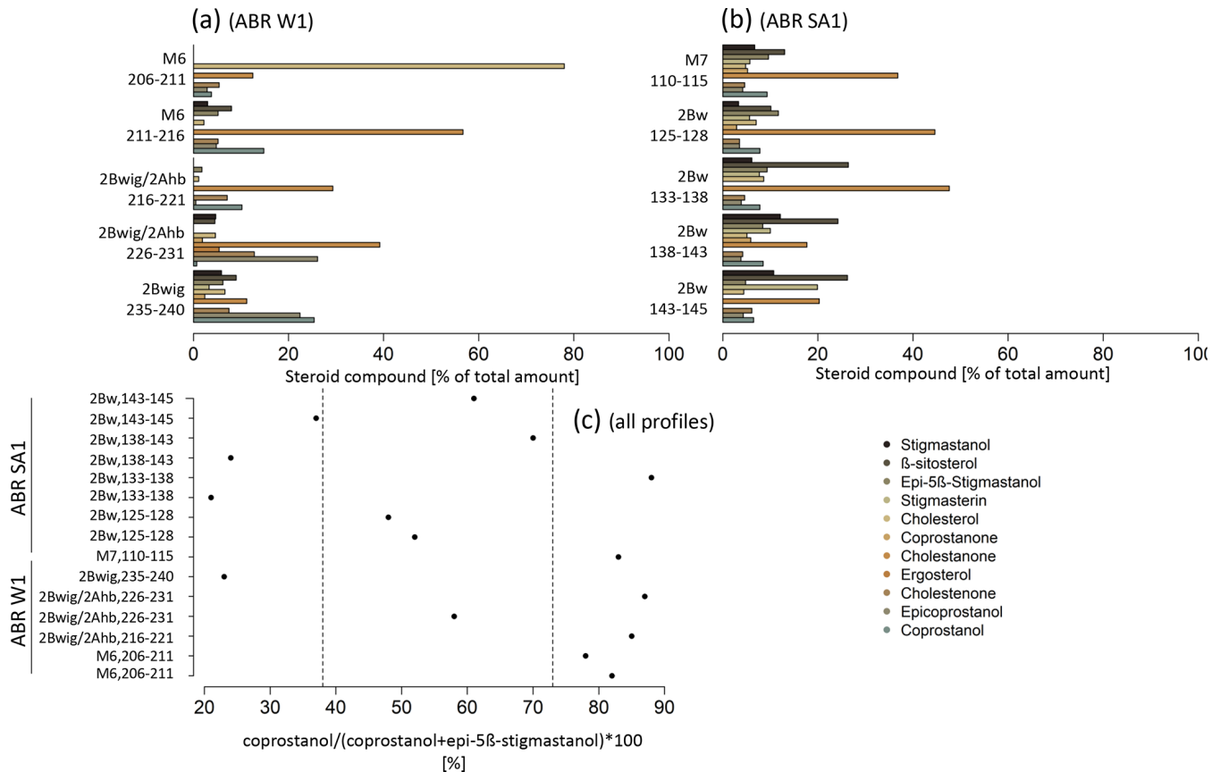
Figure 11. Steroid compounds as percent of total amount (a–b) of selected colluvial profiles and sampling depths (cm). Steroid ratio according to Leeming et al. (1997) (c). Values < 38% indicate herbivorous faeces; values > 73% indicate omnivorous faeces.
