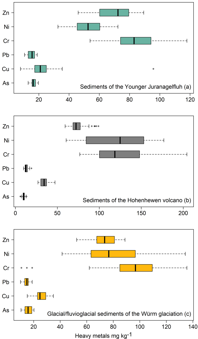
Figure 12. Heavy metal contents of the soil profiles ABR W1, ABR W2, ABR M, ABR S30, ABR SA1 and ABR SA2 according to their soil substrates: (a) sediments of the Younger Juranagelfluh ( n : 113); (b) sediments of the Hohenhewen volcano ( n : 93); (c) glacial/fluvioglacial sediments of the Würm glaciation ( n : 38). The box plots show median, 25th ( Q_1 ) to 75th ( Q_3 ) percentile (i.e., interquartile range, IQR), data minimum ( Q_1 - 1.5 \times \text{IQR} ), data maximum ( Q_3 + 1.5 \times \text{IQR} ) and outliers.
