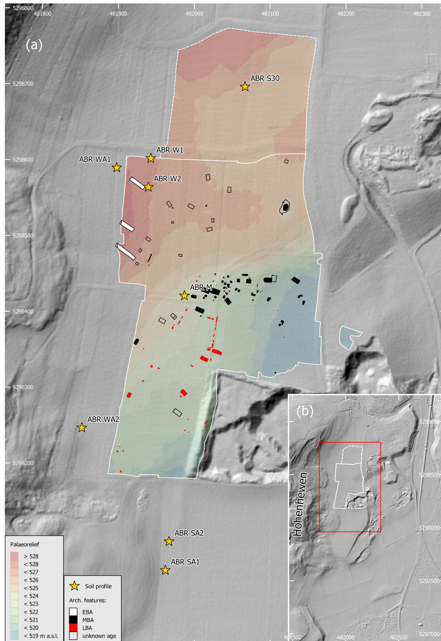
Figure 2. (a) Location of the investigated colluvial deposits and the Bronze Age structures (EBA: Early Bronze Age; MBA: Middle Bronze Age; LBA: Late Bronze Age) and their topographic situation in Anselfingen-Breite (ABR). Colored area shows boundary A according to Edgeworth et al. (2015), i.e., the paleo-surface on which the colluvial deposits accumulated. (b) The excavation area (red frame) and the ascent to the Hohenhewen to the west. Coordinates are shown in the UTM 32N reference system; EPSG 25832. Lidar credits: © LGL Baden-Württemberg; https://www.lgl-bw.de , provided on 21 November 2019 (date of recording 2002, resolution 1 × 1 m).
