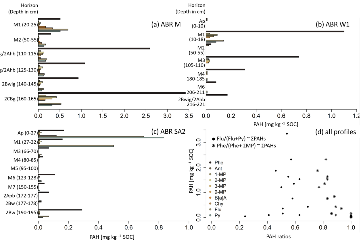
Figure 9. Polycyclic aromatic hydrocarbons (PAHs) with SOC normalization (a–c) of selected colluvial profiles and sampling depths (cm); PAH ratios vs. sum of PAHs (d). Phe: phenanthrene, Ant: anthracene, 1-MP: 1-methyl-phenanthrene, 2-MP: 2-methyl-phenanthrene, 3-MP: 3-methyl-phenanthrene, 9-MP: 9-methyl-phenanthrene, B[a]A: benz[a]anthracene, Chy: chrysene, Fl: fluoranthene, Py: pyrene.
