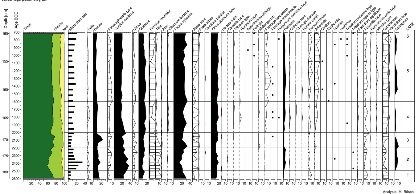
Figure 13. Pollen profile of Grassee mire. NAP: non-airborne pollen. The samples were investigated in increments of 1 cm.
