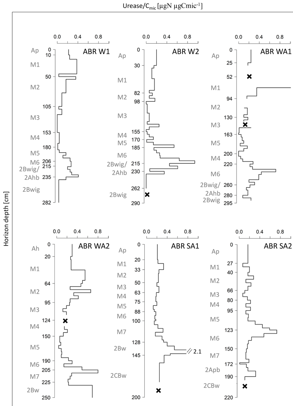
Figure 10. Depth profiles of Urease / C_{mic} ratio of selected colluvial profiles. “x”: not analyzed.
