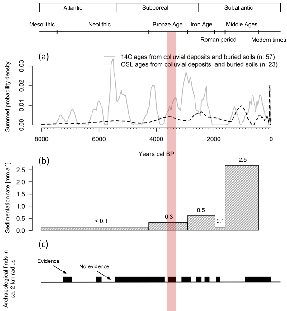
Figure 15. Summed probability density (SPD) curves from AMS ^{14}\text{C} and OSL ages (a). Sedimentation rate by depositional ages (OSL) and related to archaeological periods (b). Evidence of archaeological finds within a radius of 2 km from the Anselfingen settlement site (c). The red bar marks the Middle Bronze Age period.
