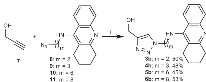
Scheme 1. Synthesis of reference compounds 3b–6b . (i) CuSO_4 \cdot 5H_2O , sodium ascorbate, DMF, RT.
