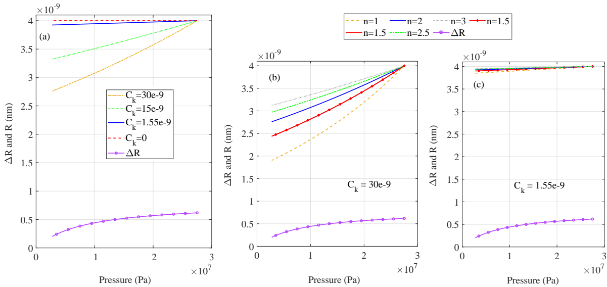
Fig. 4. Adsorbed layer thickness \Delta R(p) and pore radius R(p) vs pressure for different values of compressibility (in Pa ^{-1} ) (a), and variations of geometry parameter n for a high compressibility (b) and low compressibility (c).
