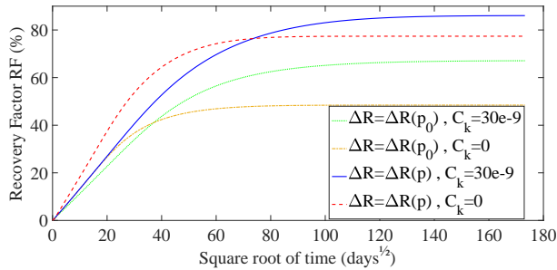
Fig. 15. Recovery factor RF vs time for four cases: Zero compressibility with desorption (red) and without desorption (orange) and high compressibility of 30 \times 10^{-9} Pa ^{-1} with desorption (blue) and without desorption (green).
