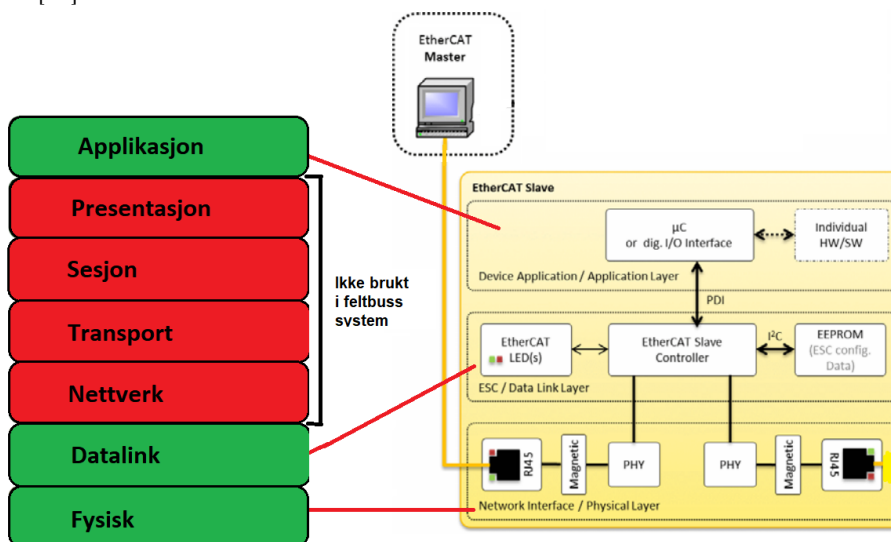
Figur 2.12: EtherCAT OSI (ref:[25], s.10)
