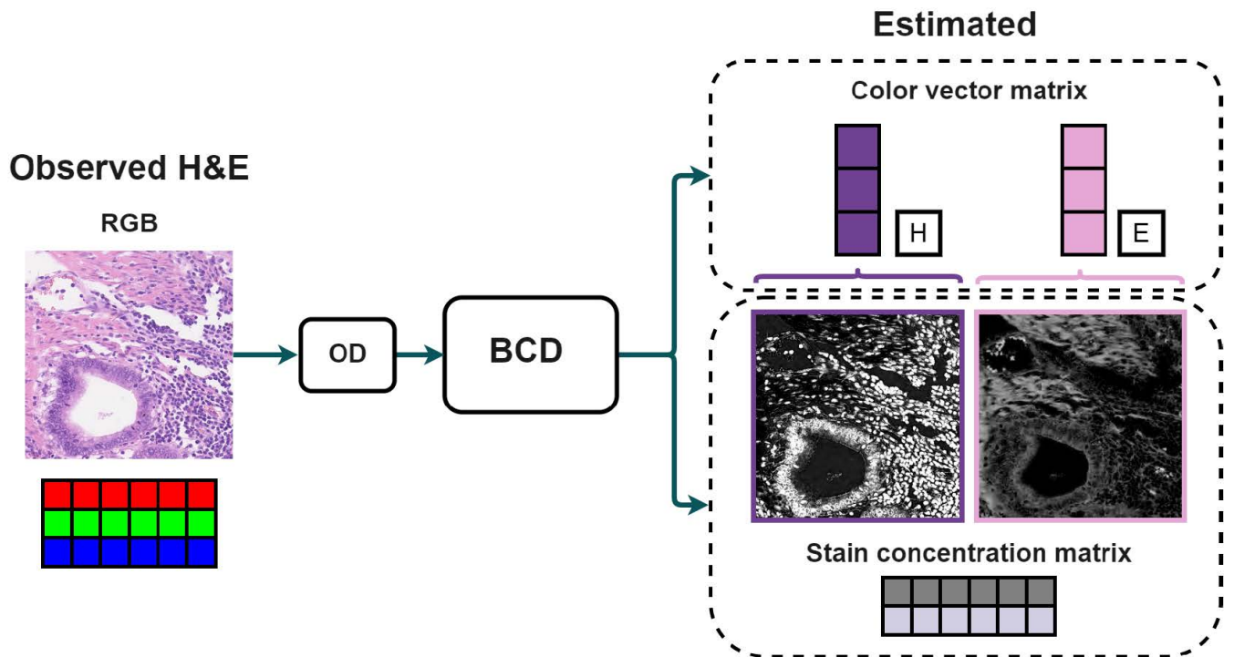
FIGURE 7. Usual pipeline for stain separation using BCD. First, the RGB image which can be seen as a matrix with one row for each RGB channel, is transformed to the logarithmically inverted OD space. Then, different methods are used to separate color from structure. The outputs are the estimated color vector matrix and stain concentration matrix, which contain the color information for each stain (H&E in the example) and the concentration of each stain for each pixel, respectively. The concentration matrix can be seen in the figure with one row for each stain as well as a grayscale image for each stain.
