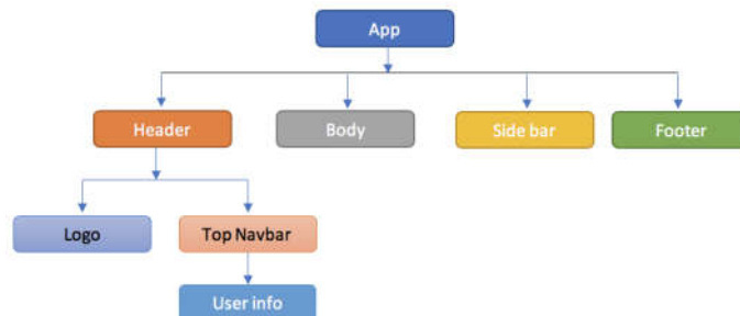
Figure 3.4: React component architecture [10]
