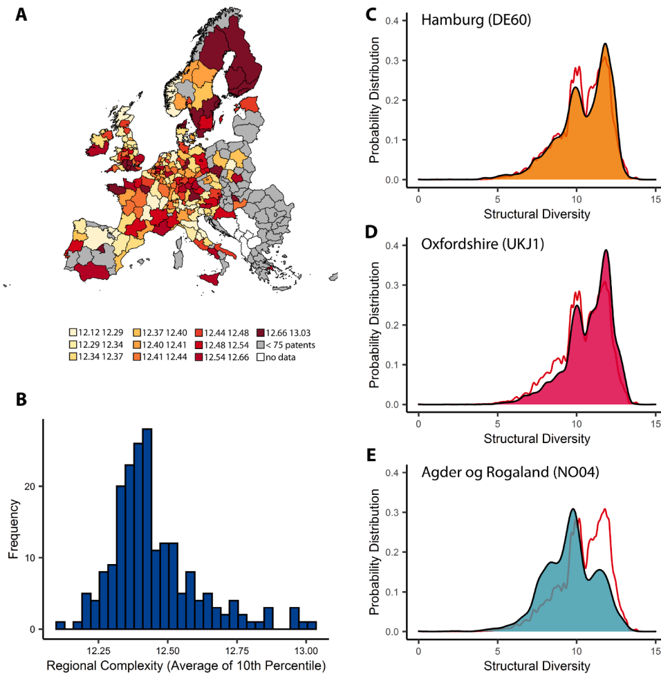
Fig. 3. Technological complexity in Europe between 2000 and 2014. A Map and B distribution of regional complexity scores across all regions. Patents' complexity distribution in all regions (red line) compared with three selected regions C urban region (Hamburg, Germany), D technology-intensive region (Oxfordshire, United Kingdom), and E resource-intensive region (Agder og Rogaland, Norway). (For the interpretation of the colors in the figure, the reader is referred to the web version of this article.)
