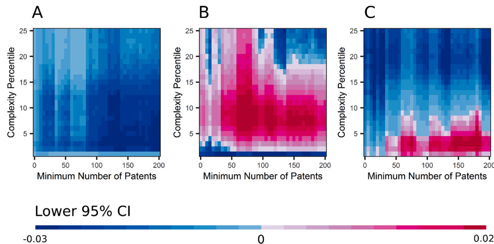
Fig. 5. Robustness analysis with alternative complexity percentiles (ranging between top 1% and top 25% complex activities) and minimum patent numbers (ranging between 0 and 200 patents). Lower 95% confidence intervals are based on OPM estimations. Pink colors indicate that the lower boundary of the confidence intervals excludes values equal to and smaller than zero. rcpx is lagged by A 3 years, B 4 years and C 5 years.
