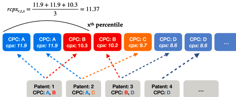
Fig. 2. Aggregation of technological complexity at the regional level.
