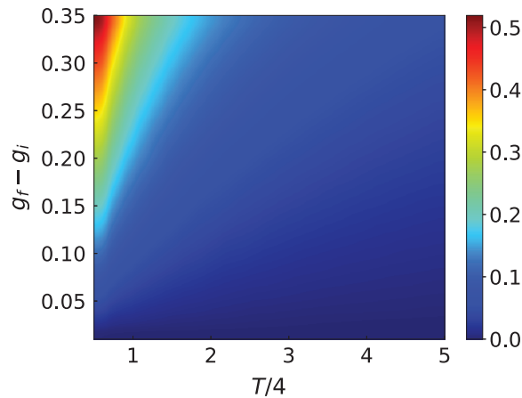
Fig. 4. Plot of the effective temperature of the steady state as a function of T and (g_f - g_i)/g_c , for a fixed g_i/g_c = 0.1 . The plot shows that the effective temperature increases with decreasing T and increasing drive amplitude. See text for details.
