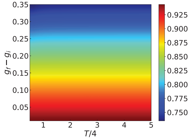
Fig. 2. Plot of the steady state value of \rho as a function of the drive amplitude (g_f - g_i)/g_c and ramp time T , for g_i/g_c = 0.1 . The plot shows \rho to be a monotonically decreasing function of the drive amplitude for any T in the ordered phase. See text for details.
