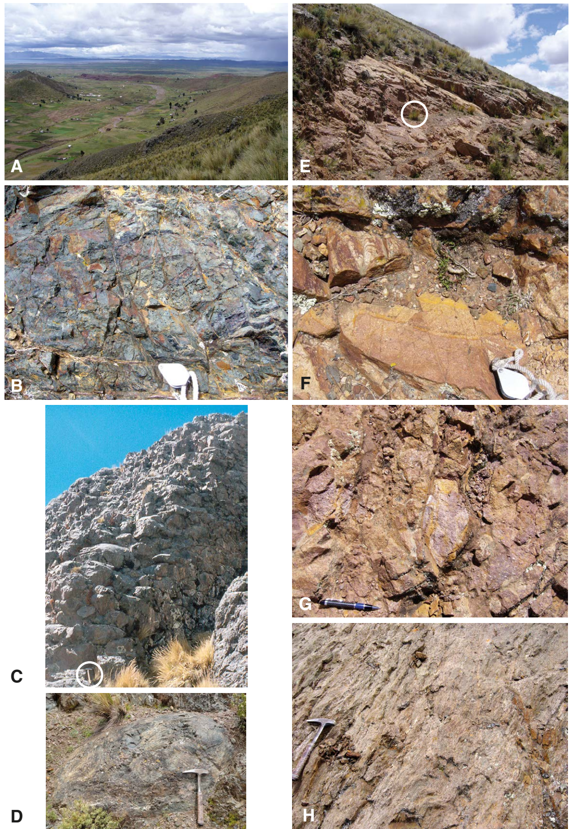
Figure 5. Outcrops and lithologies at Cerro Chilla (Altiplano, Bolivia). (A) Overview toward the north; Lake Titicaca in the distance; 16°37'46.03" S, 68°40'12.63" W. (B) Vesicular basalt lava; 16°40'09.25" S, 68°45'00.78" W. (C) Succession of pillowed basalt; 16°41'21.78" S, 68°43'46.24" W. Circle highlights a hammer for scale. (D) Detail of pillowed basalt; 16°37'46.93" S, 68°40'12.63" W. (E) Succession of sandstones; 16°40'19.53" S, 68°44'55.30" W. Circle marks 40 cm high Peruvian feathergrass ( Jarava ichu ). (F) Detail of sandstone; 16°40'22.85" S, 68°44'49.07" W. (G) Conglomerate; 16°40'22.85" S, 68°44'49.07" W. (H) Tuffaceous phyllite; 16°40'24.45" S, 68°44'37.34" W.
