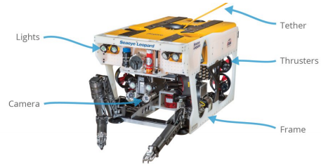
Figure 1.16: Diagram of common components
