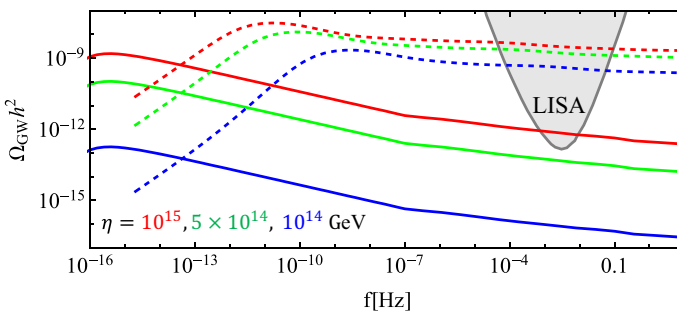
Fig. 16 SGWB spectrum from a global (solid) and gauge (dashed) string network in standard cosmology with loop length parameter \alpha = 0.1 , and symmetry breaking scale \eta = 10^{15}, 5 \times 10^{14}, 10^{14} GeV for red, green, blue, respectively. The grey region is the LISA sensitivity
