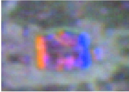
(a) SAR RGB response of settlement mound. (b) Optical image of same settlement mound.
