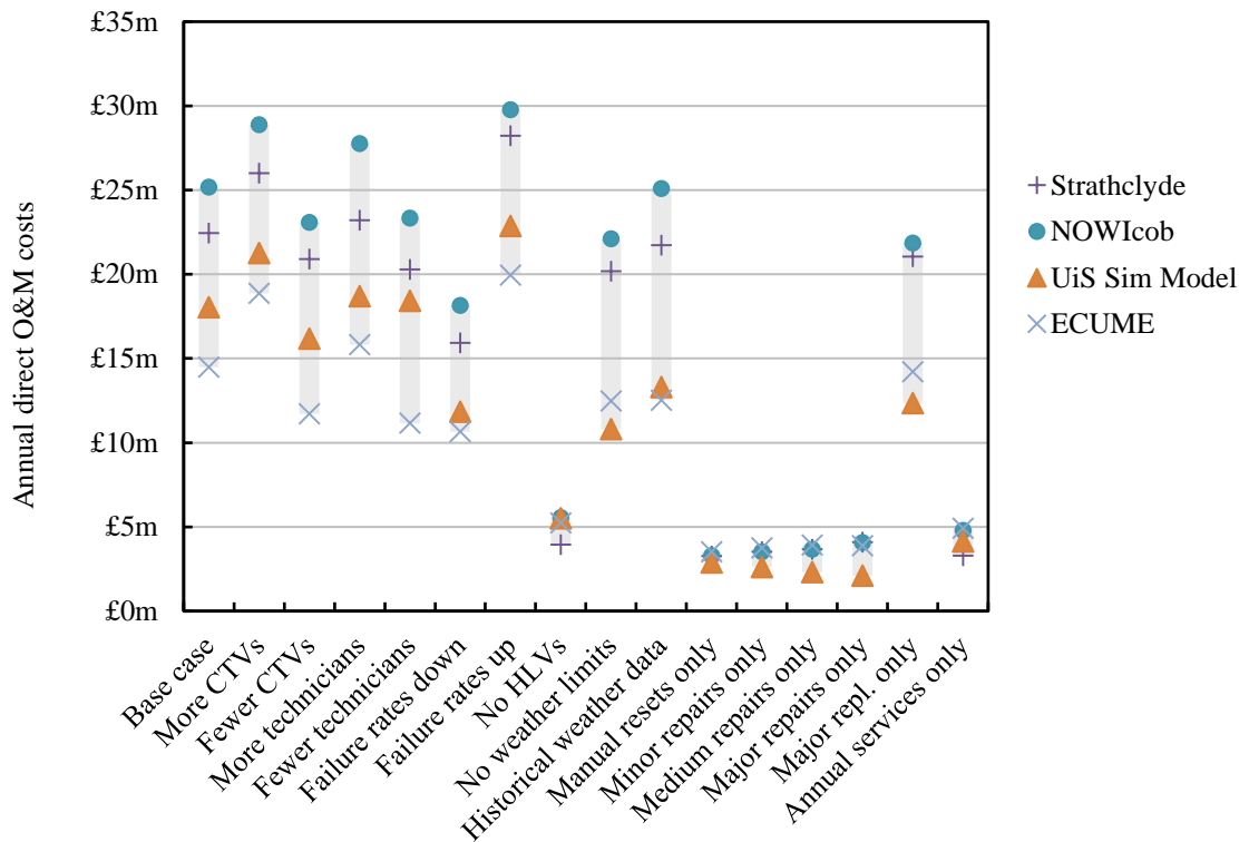
Figure 2 Average values for the average annual direct O&M costs for the models for the reference cases
