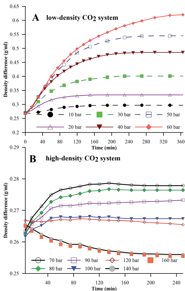
Fig. 5 Density differences between the HD and the environment for the pressure ranges of 0 to 60 bar (A) (low-density \text{CO}_2 ) and 70 to 160 bar (B) (high-density \text{CO}_2 ) at 25 °C.
