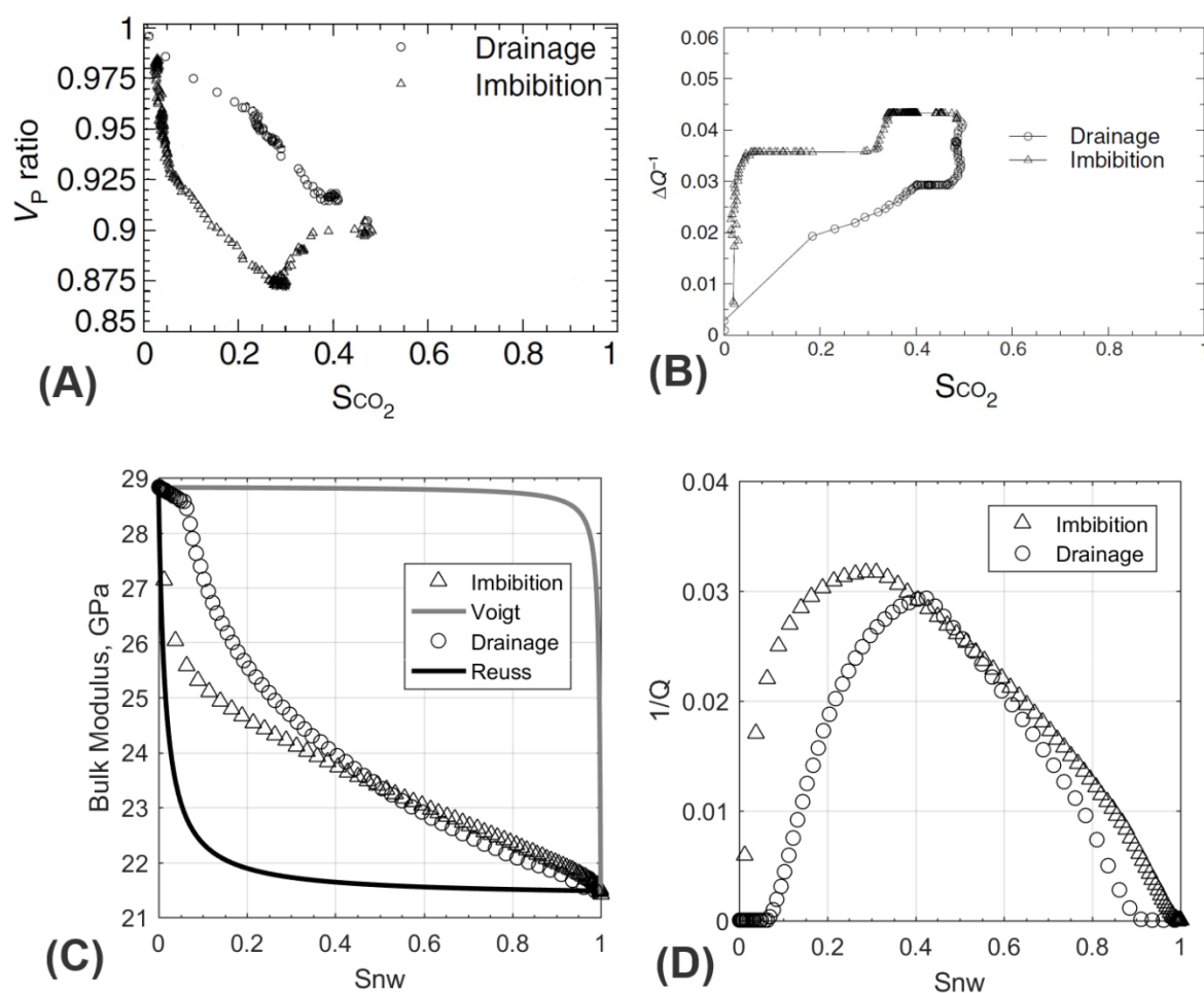
Figure 13. (A) and (B) Laboratory measurements of P-wave velocity and its attenuation on low-permeability sandstone during drainage (CO 2 injection) and imbibition (brine injection) (Modified after Zhang et al. , 2015). (C) and (D) calculated bulk moduli and attenuation hysteresis during drainage and imbibition, see Table 1 for input parameters and Figure 14 for “inkbottle” effect during drainage and imbibition. Horizontal scale in (A) and (B) shows gas saturation of the core sample, while in (C) and (D) shows gas saturation of the crack. Both experimental and numerical results predict higher velocity and bulk moduli during drainage and lower attenuation during drainage at gas saturations below 50%.
