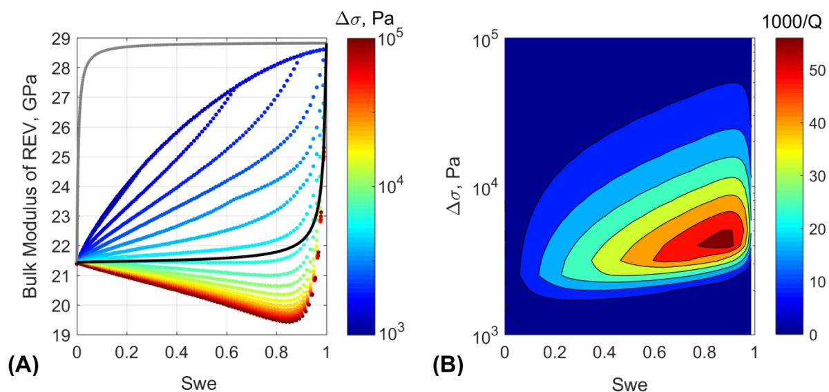
Figure 12. (A) Bulk Modulus of REV vs wetting phase saturation, calculated for different magnitudes of wave induced stress perturbation, shown on the colour-scale. Grey and black curves show Voigt and Reuss upper and lower bounds. (B) Attenuation \frac{1000}{Q} factor is shown on the colour scale, as a function of wave-induced stress perturbation magnitude and wetting phase saturation, shown on abscissa and ordinate, respectively. See Tables 1 and 2 for input parameters for Case 4 (Wettability effect).
