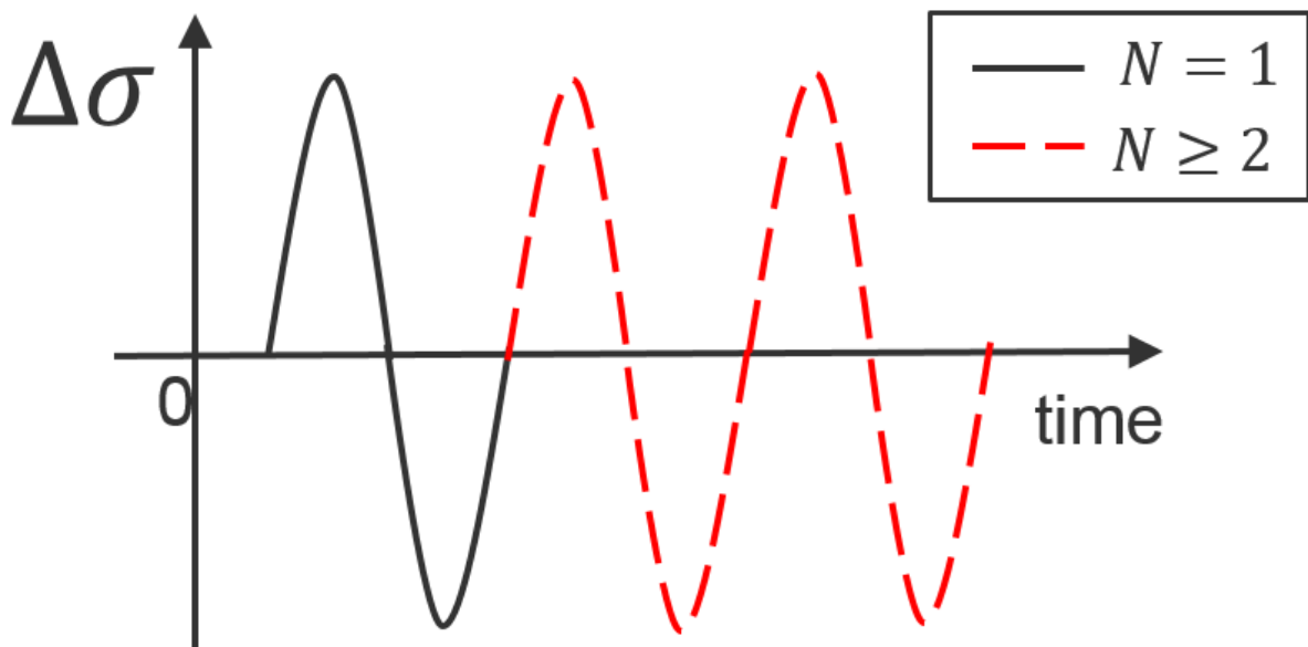
Figure 5. Periodic stress perturbation, acting on the external boundary of REV. The first cycle ( N = 1 ) is shown by continuous black curve; subsequent cycles are shown by the red dashed curve.
