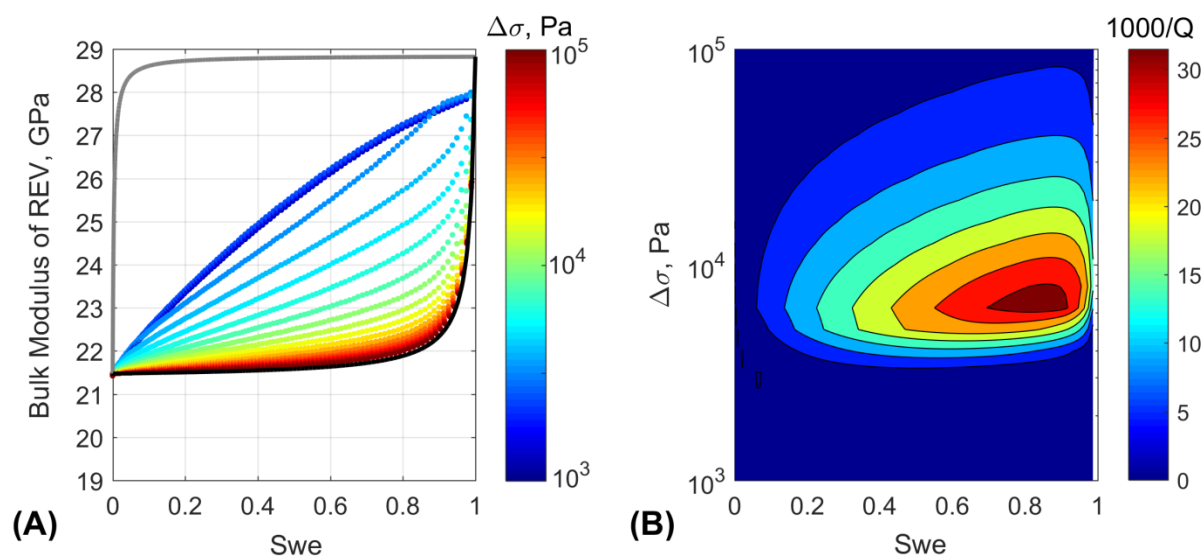
Figure 10. (A) Bulk Modulus of REV vs wetting phase saturation, calculated for different magnitudes of wave induced stress perturbation, shown on the colour-scale. Grey and black curves show Voigt and Reuss upper and lower bounds. (B) Attenuation \frac{1000}{Q} factor is shown on the colour scale, as a function of wave-induced stress perturbation magnitude and wetting phase saturation, shown on abscissa and ordinate, respectively. See Tables 1 and 2 for input parameters for Case 2 (Frequency effect).
