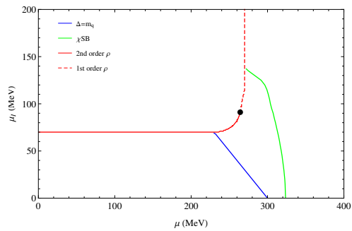
FIG. 2. Phase diagram in the \mu - \mu_I plane at the physical point in the homogeneous case at T = 0 . See main text for details.
