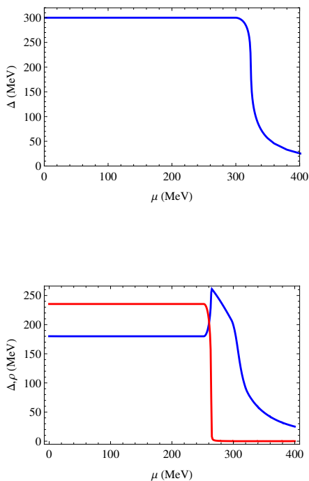
FIG. 3. Chiral condensate (blue line) and pion condensate (red line) as functions of the chemical potential \mu for \mu_I = 0 (upper panel) and \mu_I = 90 MeV (lower panel) at the physical point and T = 0 .
