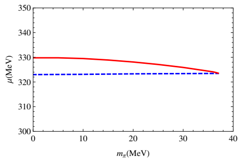
FIG. 4. Lower and upper limits of the chemical potential \mu where an inhomogeneous phase exists as a function of m_\pi for \mu_I = 0 .
