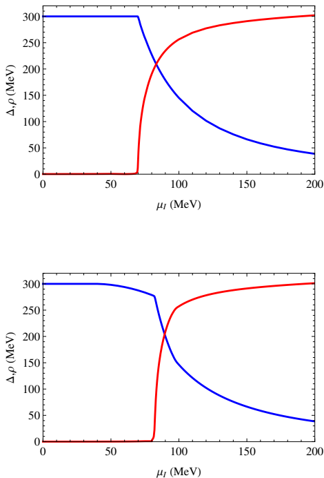
FIG. 1. Chiral condensate (blue line) and pion condensate (red line) as functions of the isospin chemical potential \mu_I for \mu = 0 (upper panel) and \mu = 260 MeV (lower panel) at the physical point and T = 0 .
