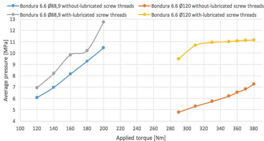
Figure 17. The average pressure of Bondura® 6.6 PINs with & without-lubricated screw threads
