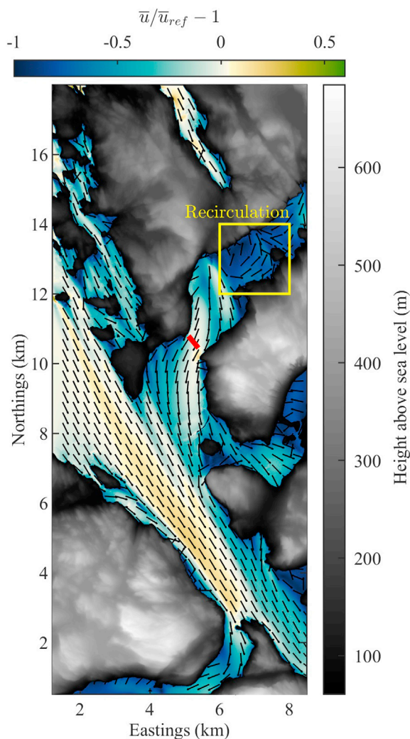
Fig. 14. Normalized mean horizontal wind velocity 60 m above the surface, simulated with a direction of 335^\circ at the inlet boundary.
