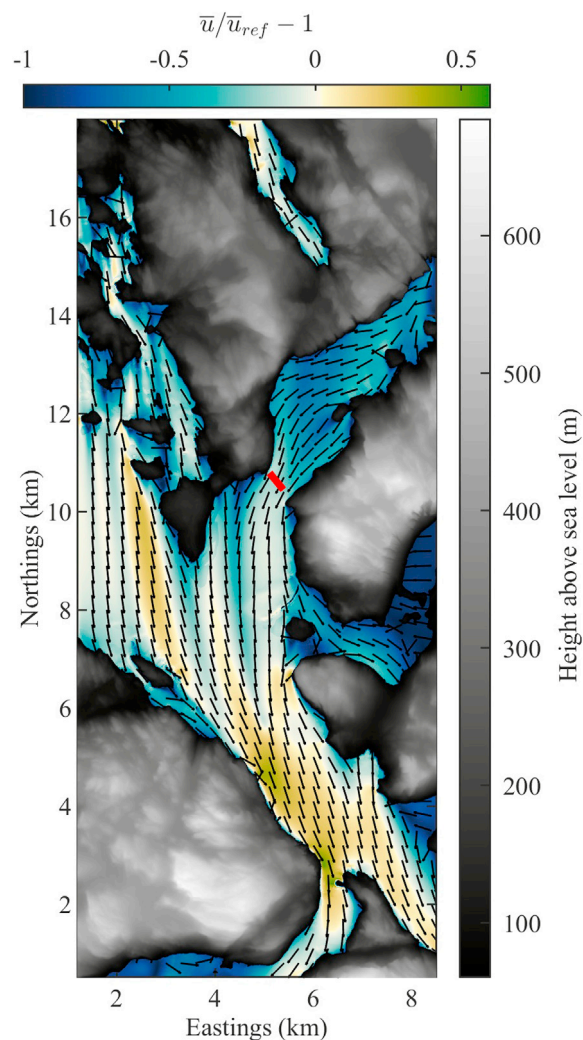
Fig. 15. Normalized mean horizontal wind velocity 60 m above the surface, simulated with a direction of 355^\circ at the inlet boundary.
