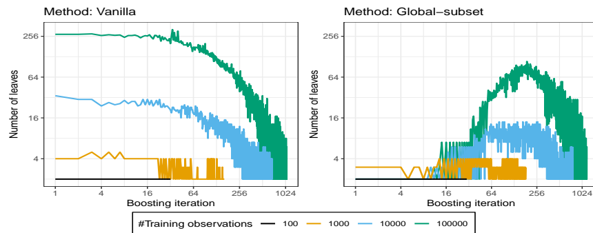
Figure 5: The number of leaves for the k 'th tree (boosting iteration k ) for different agtb models trained on the Higgs data with a varying number of training observations. Notice the log scale on both the vertical and horizontal axes.
