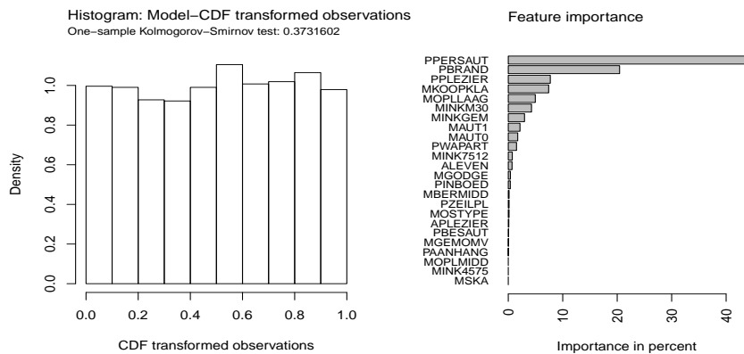
Figure 3: [left] Histogram generated by gbt.kstest , where test-response observations are transformed using (20). As the histogram closely resembles the histogram of standard uniformly distributed random variables, the model should not be discarded, something also indicated by the formal Kolmogorov-Smirnov test. [right] Feature importance plot generated by gbt.importance .
