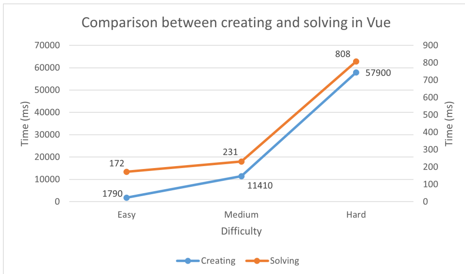
Figure 5.8: The time duration for creating and solving a Sudoku board in the Vue application.
