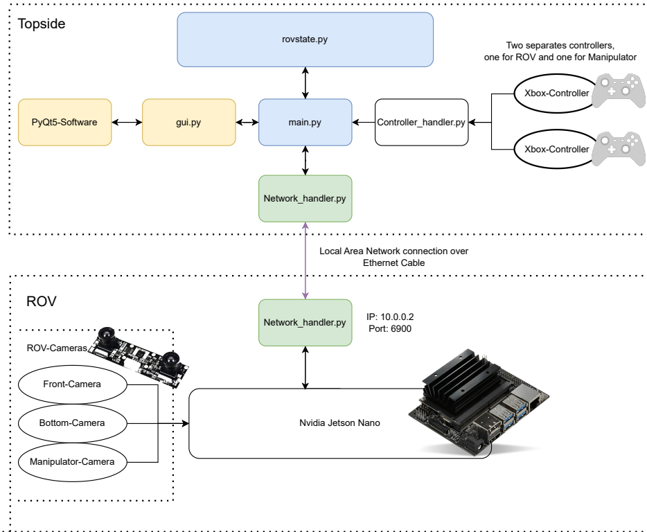
Figure 3.1: Communication structure between topside and ROV.
