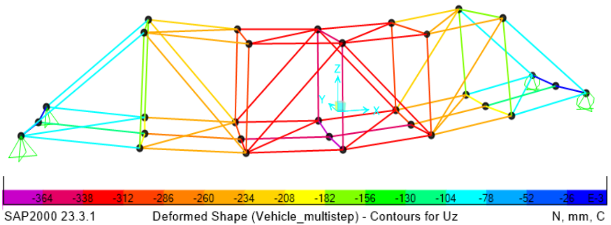
Figure 35: Deformation (Uz) results 3D dynamic analysis from SAP2000
