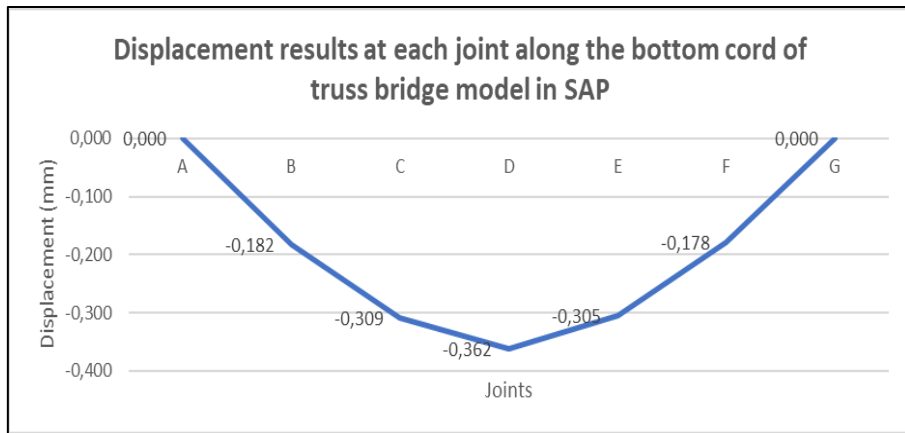
Figure 34 Displacement results from SAP multi-step analysis at each joint of the bottom cords
