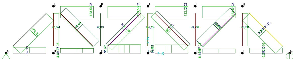
Figure 36: Dynamic 3D- member forces from SAP2000
