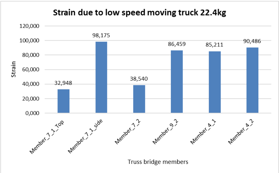
Figure 47: Max-strain at truss members due to low speed moving truck.
