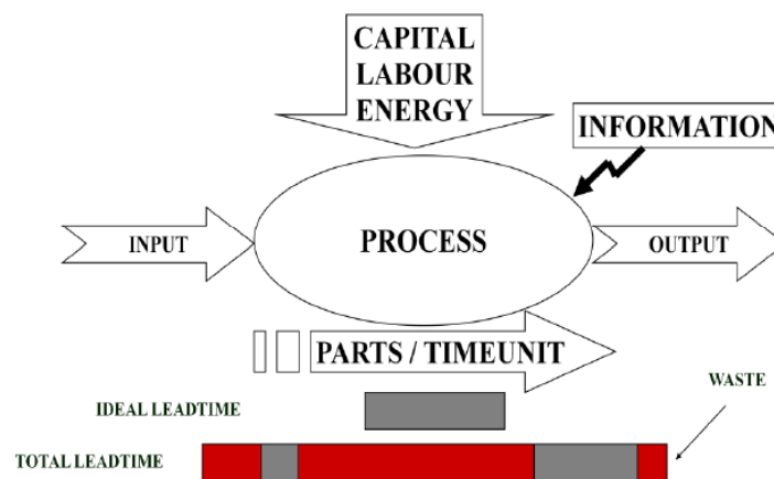
Figure 27 Process Model.[84]
